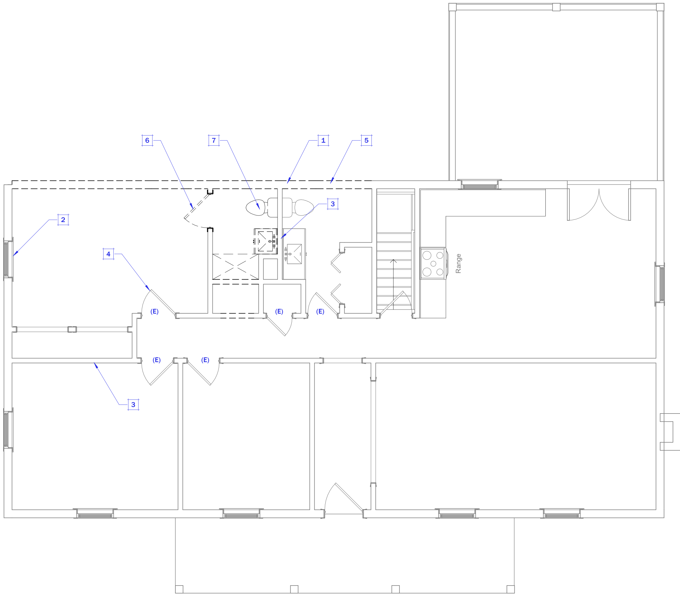
1 MAIN LEVEL DEMO PLAN 1/4" = 1'-0"
