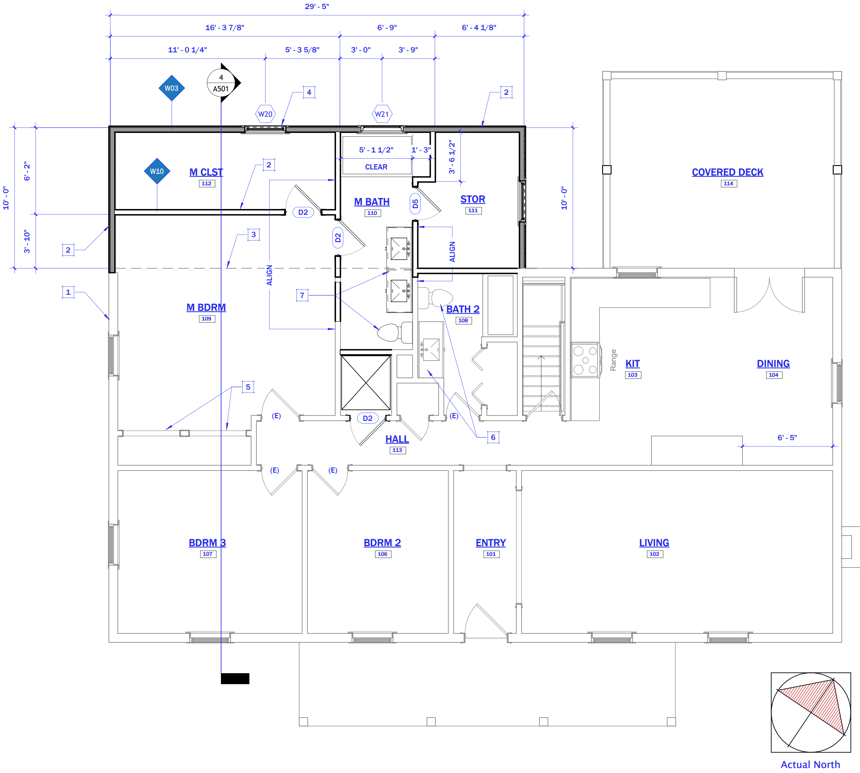
1 MAIN LEVEL FLOOR PLAN 1/4" = 1'-0"
