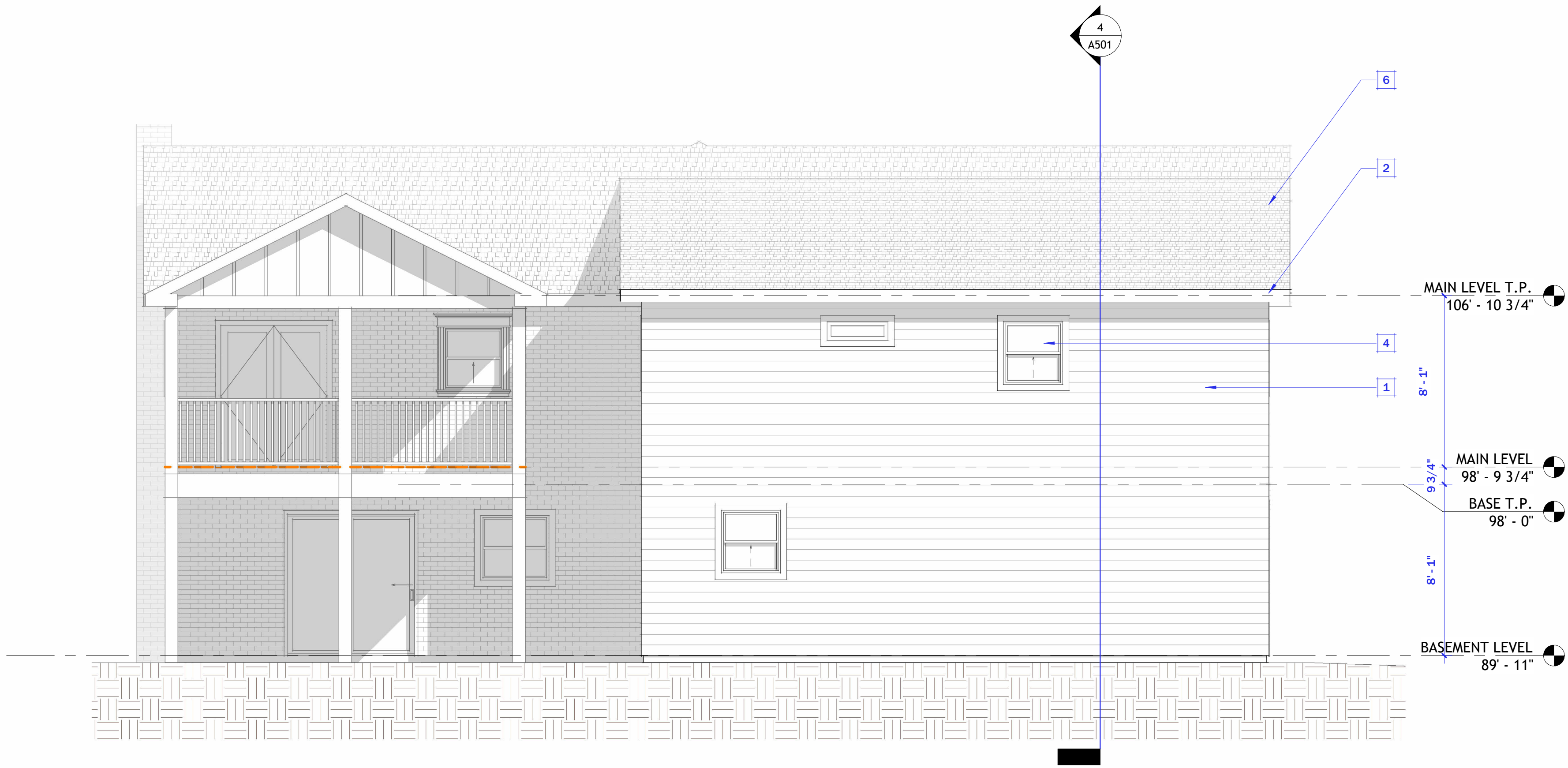
2 EAST EXTERIOR ELEVATION 1/4" = 1'-0"
