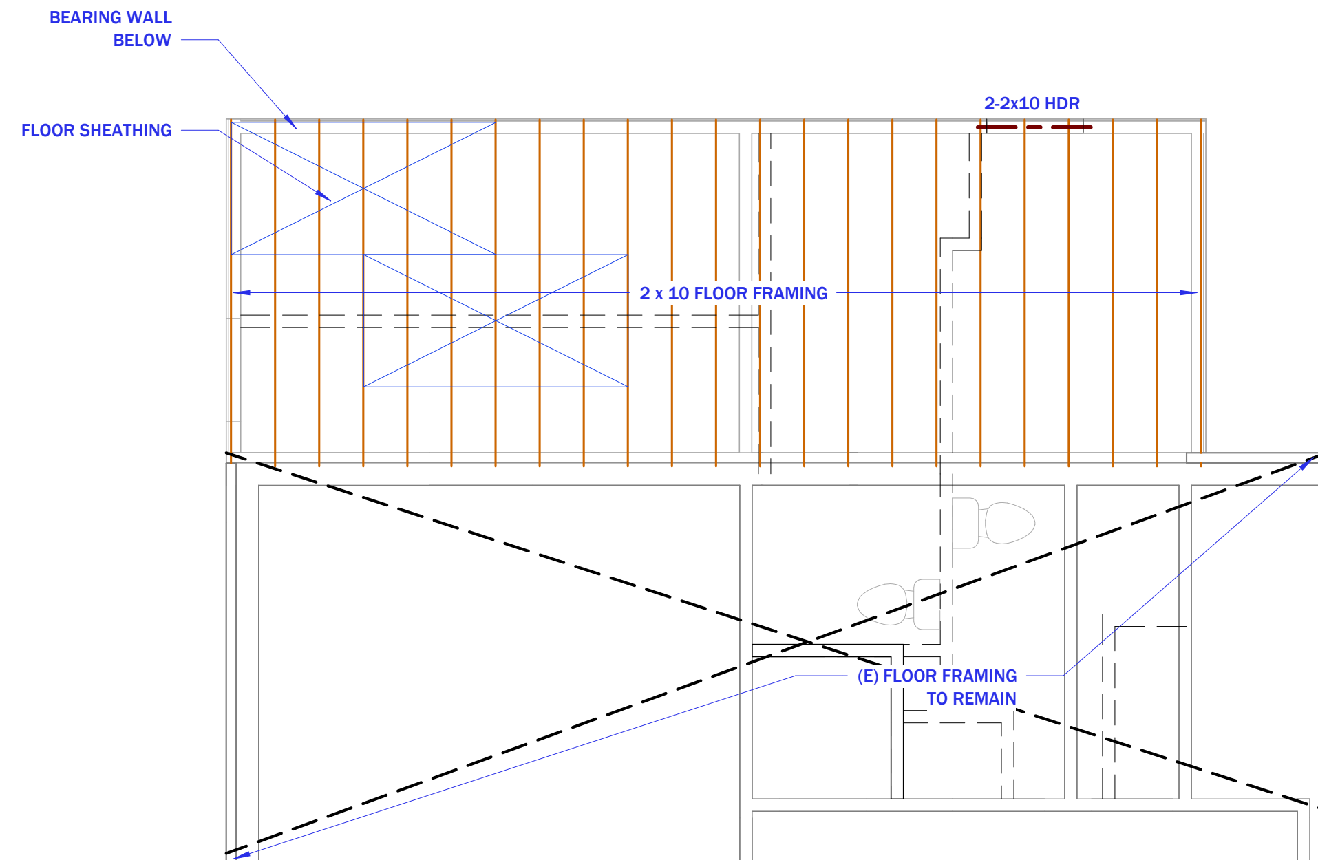
2 MAIN LEVEL FRAMING PLAN 1/4" = 1'-0"
