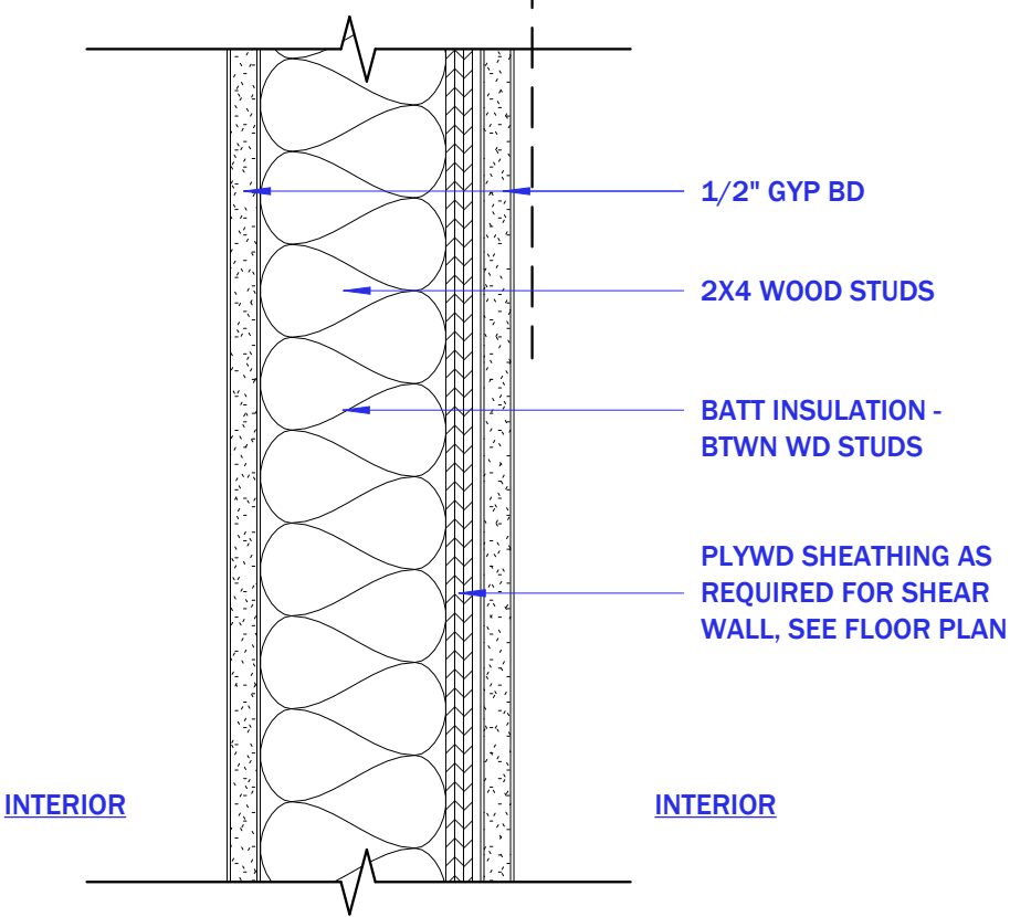
44 WALL TYPE - W10 3" = 1'-0"
