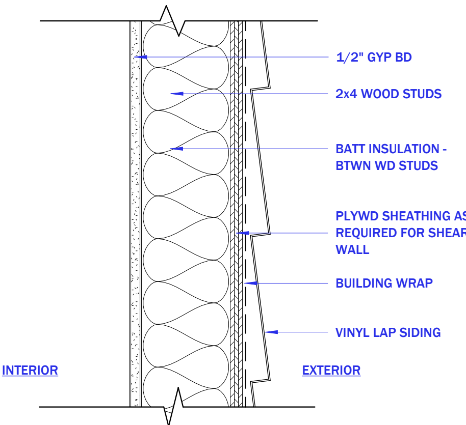
43 WALL TYPE - W03 3" = 1'-0"
