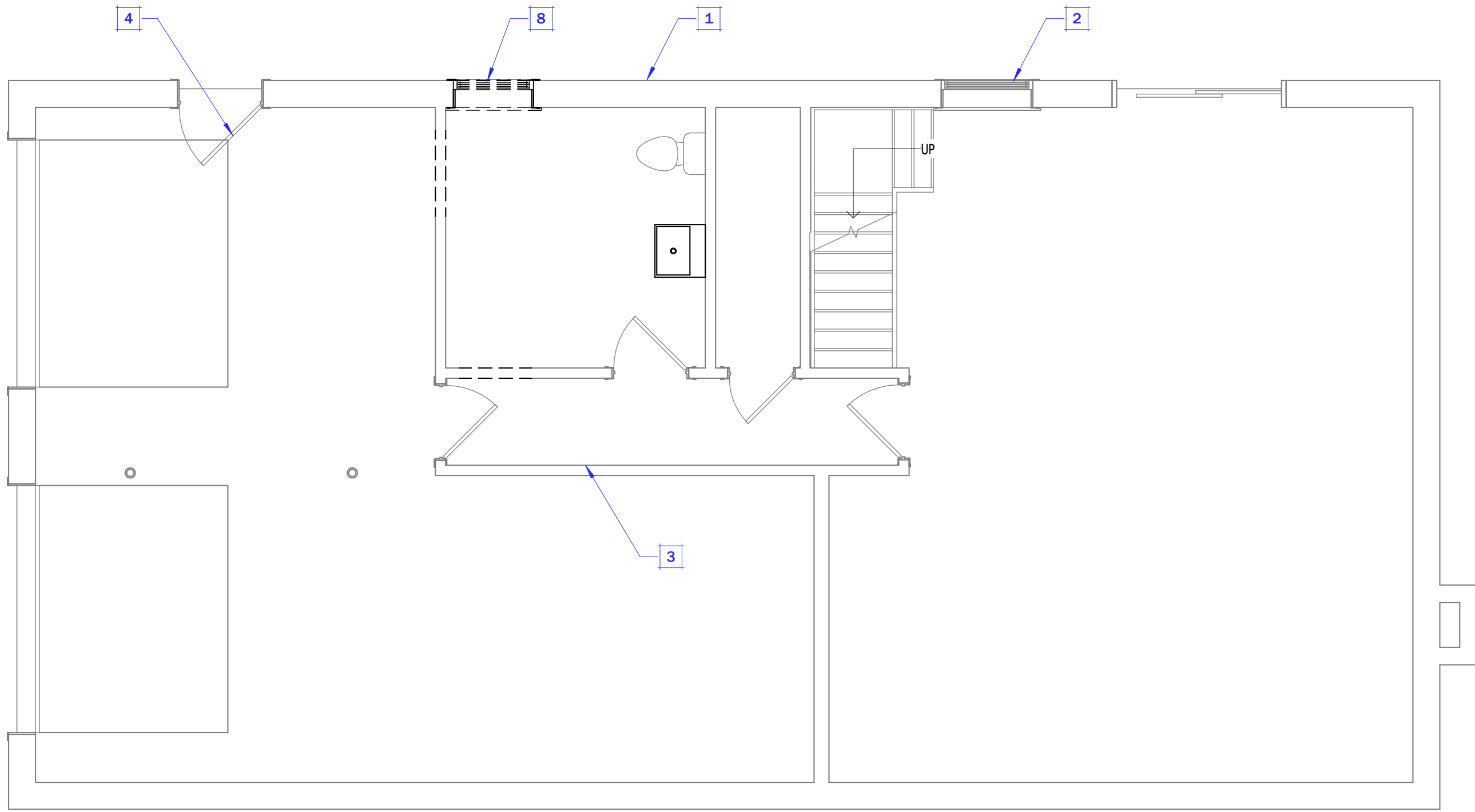
2 BASEMENT DEMO PLAN 1/4" = 1'-0"
