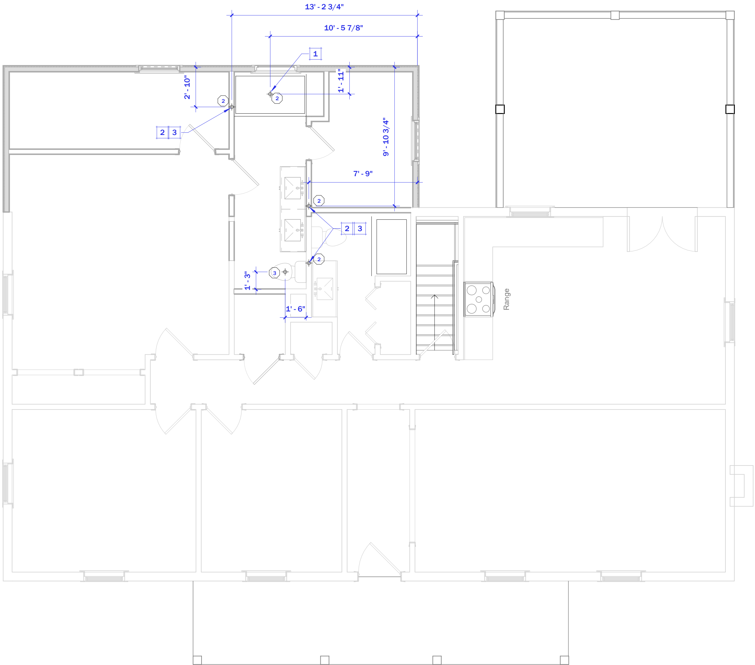
1 MAIN PLUMBING PLAN 1/4" = 1'-0"
