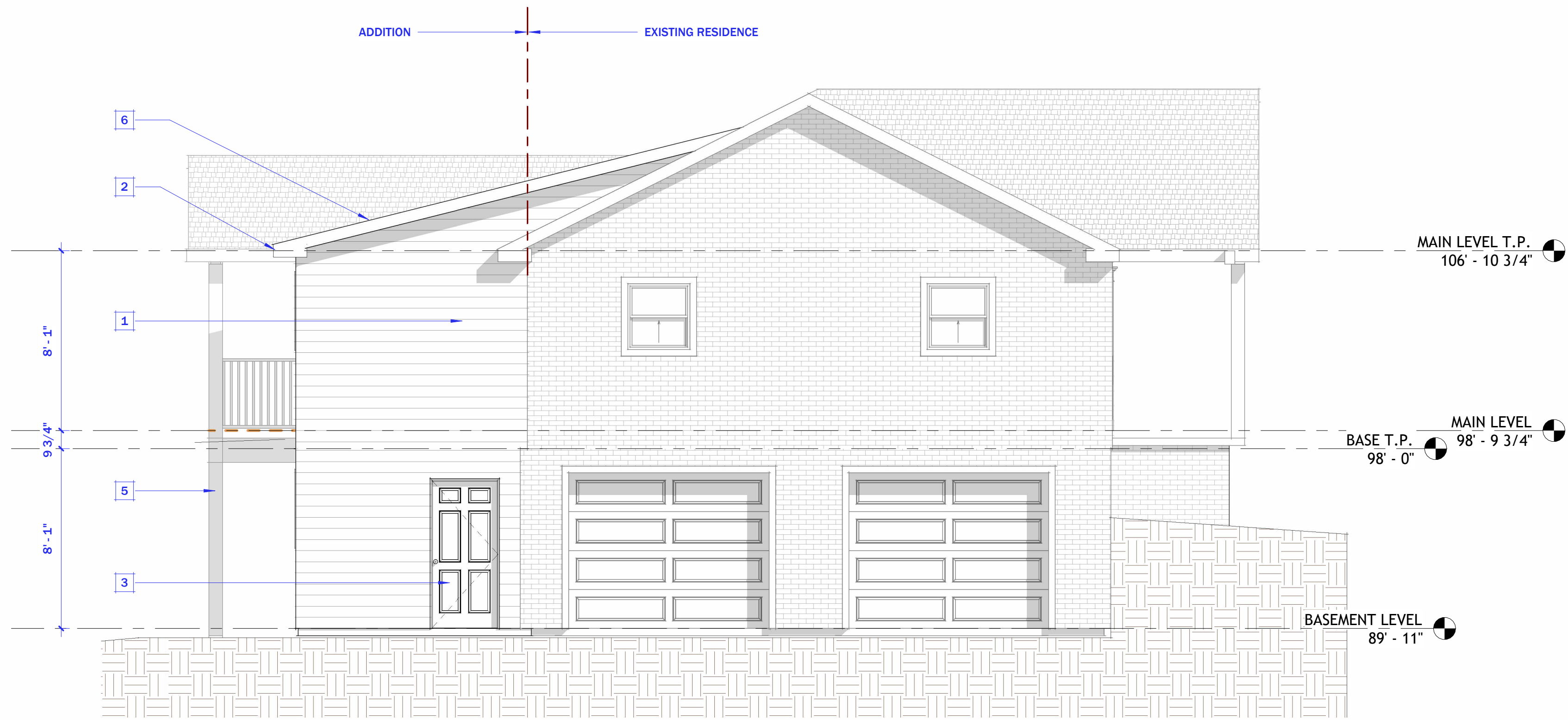
1 NORTH EXTERIOR ELEVATION 1/4" = 1'-0"
