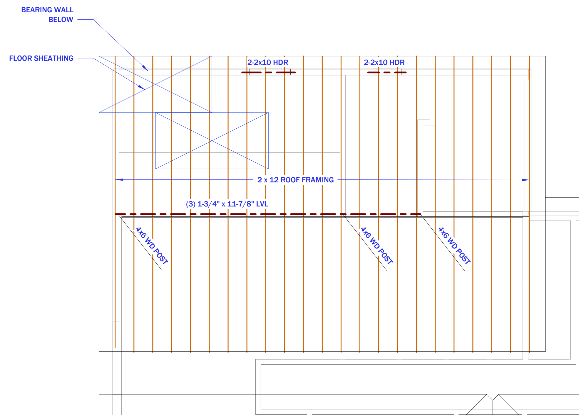
3 MAIN LEVEL ROOF FRAMING PLAN 1/4" = 1'-0"
