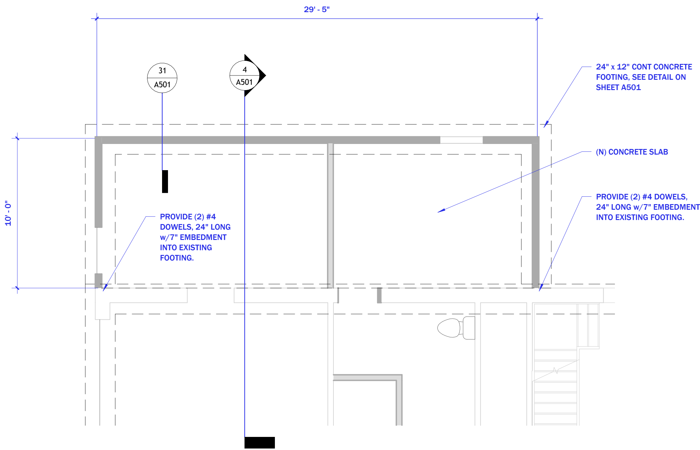
1 BASEMENT FOUNDATION PLAN 1/4" = 1'-0"
